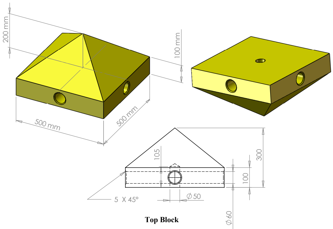
Figure 11: Specifications of the Pyramids Building Blocks
